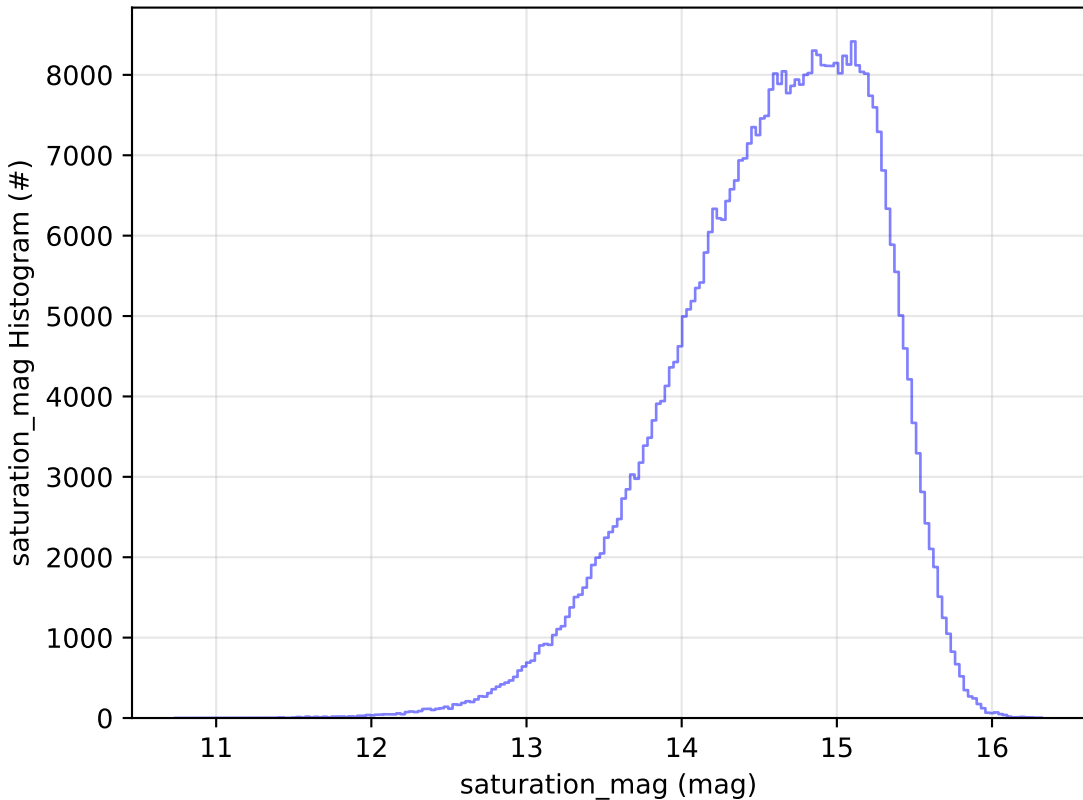
noroll_v3.4_10yrs All sky r band: saturation_mag Histogram
