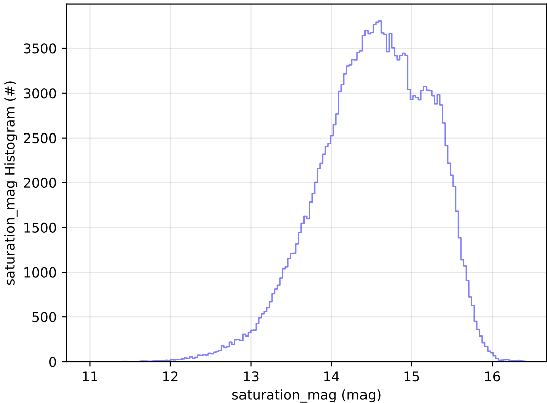
noroll_v3.4_10yrs All sky g band: saturation_mag Histogram
