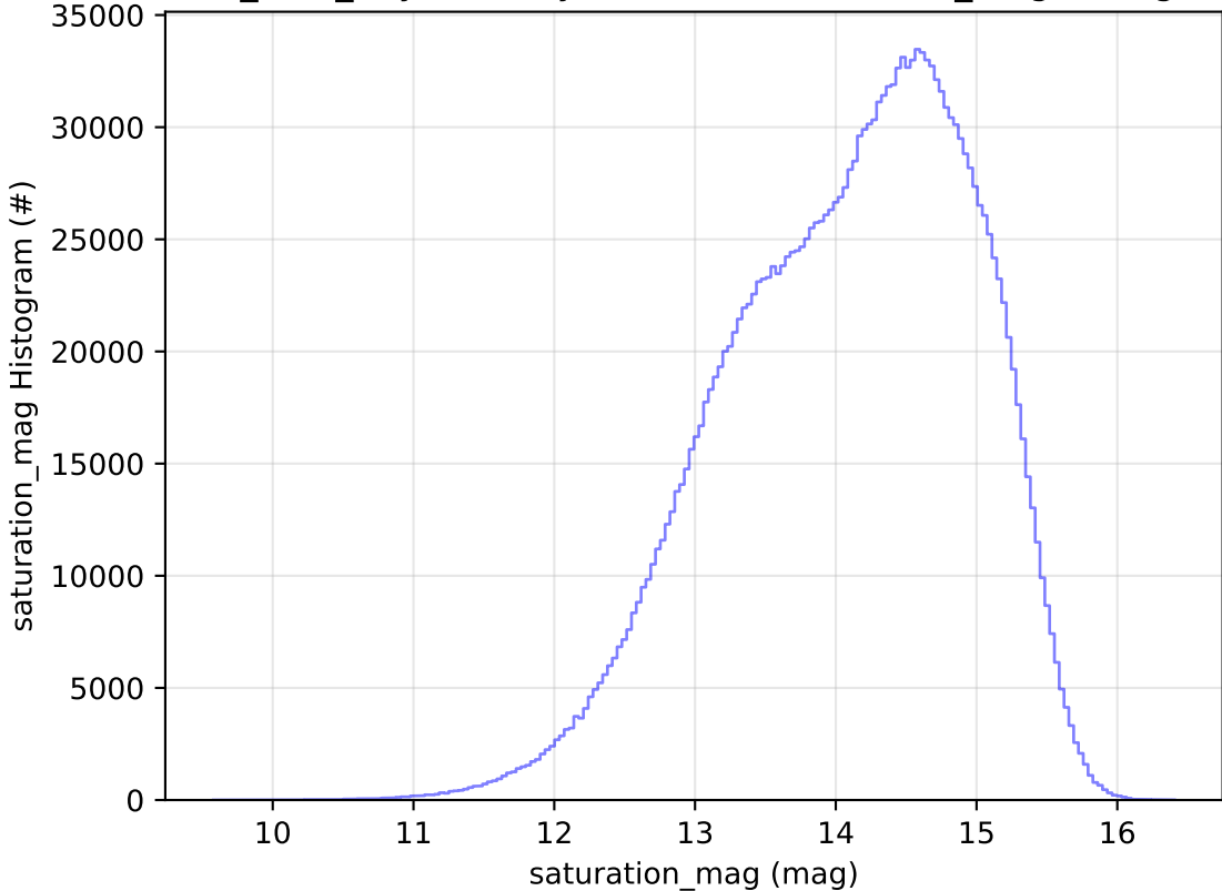
noroll_v3.4_10yrs All sky all bands: saturation_mag Histogram
