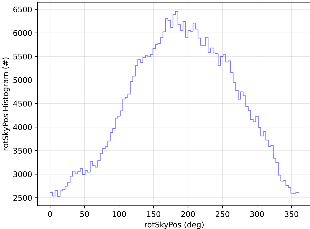
noroll_v3.4_10yrs WFD z band: rotSkyPos Histogram
