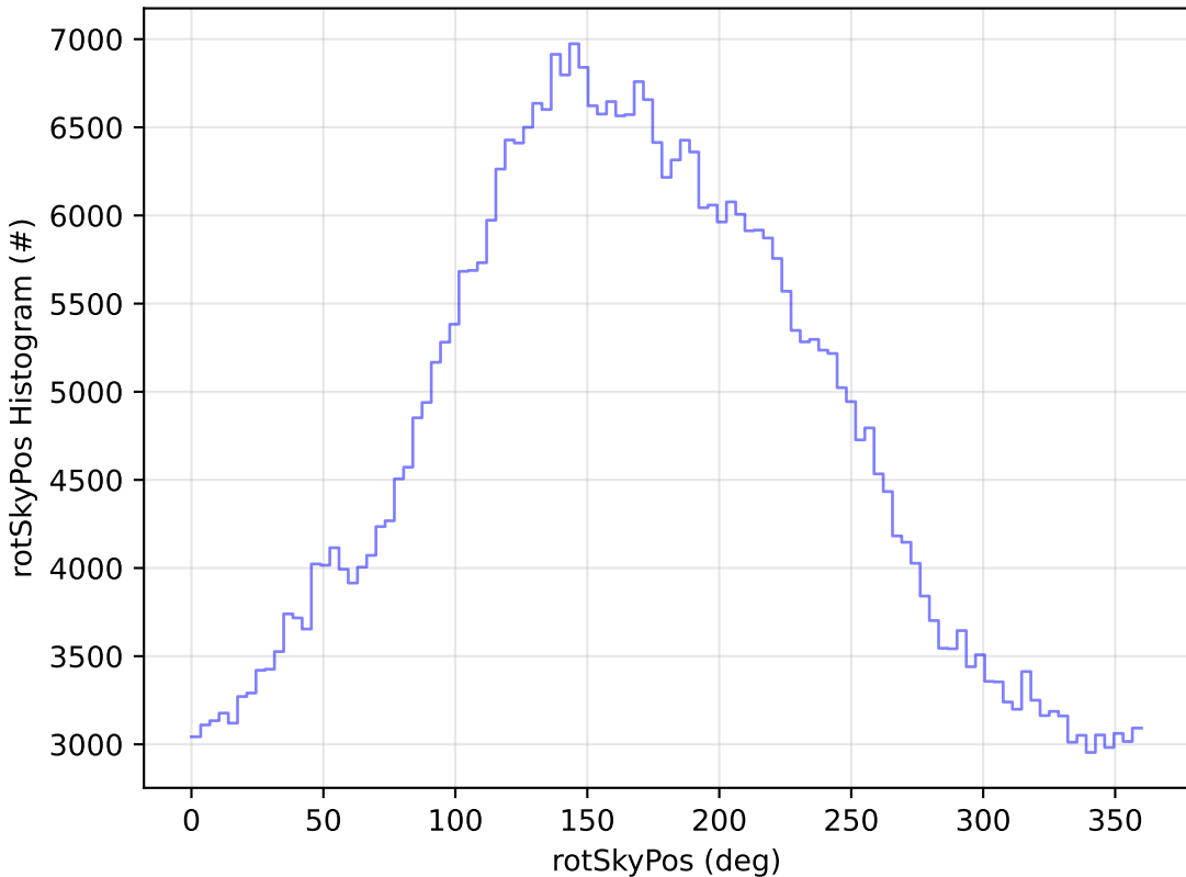
noroll_v3.4_10yrs WFD r band: rotSkyPos Histogram
