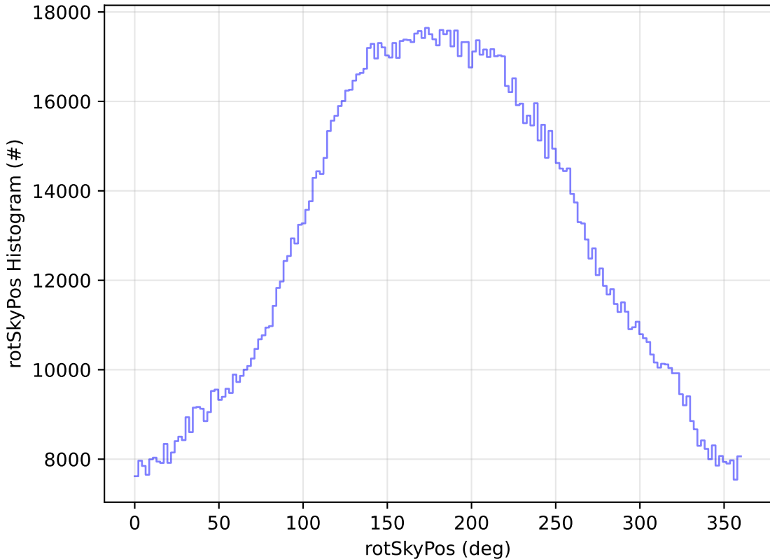
noroll_v3.4_10yrs WFD all bands: rotSkyPos Histogram
