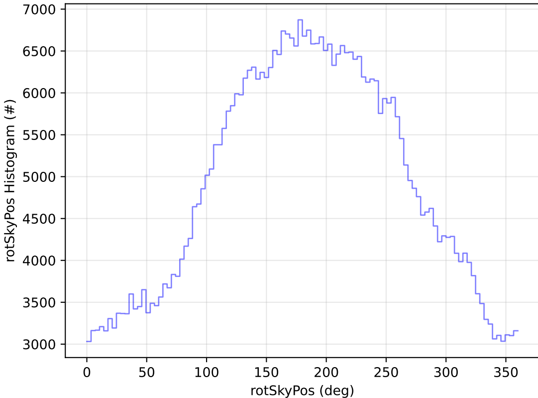
noroll_v3.4_10yrs All sky i band: rotSkyPos Histogram
