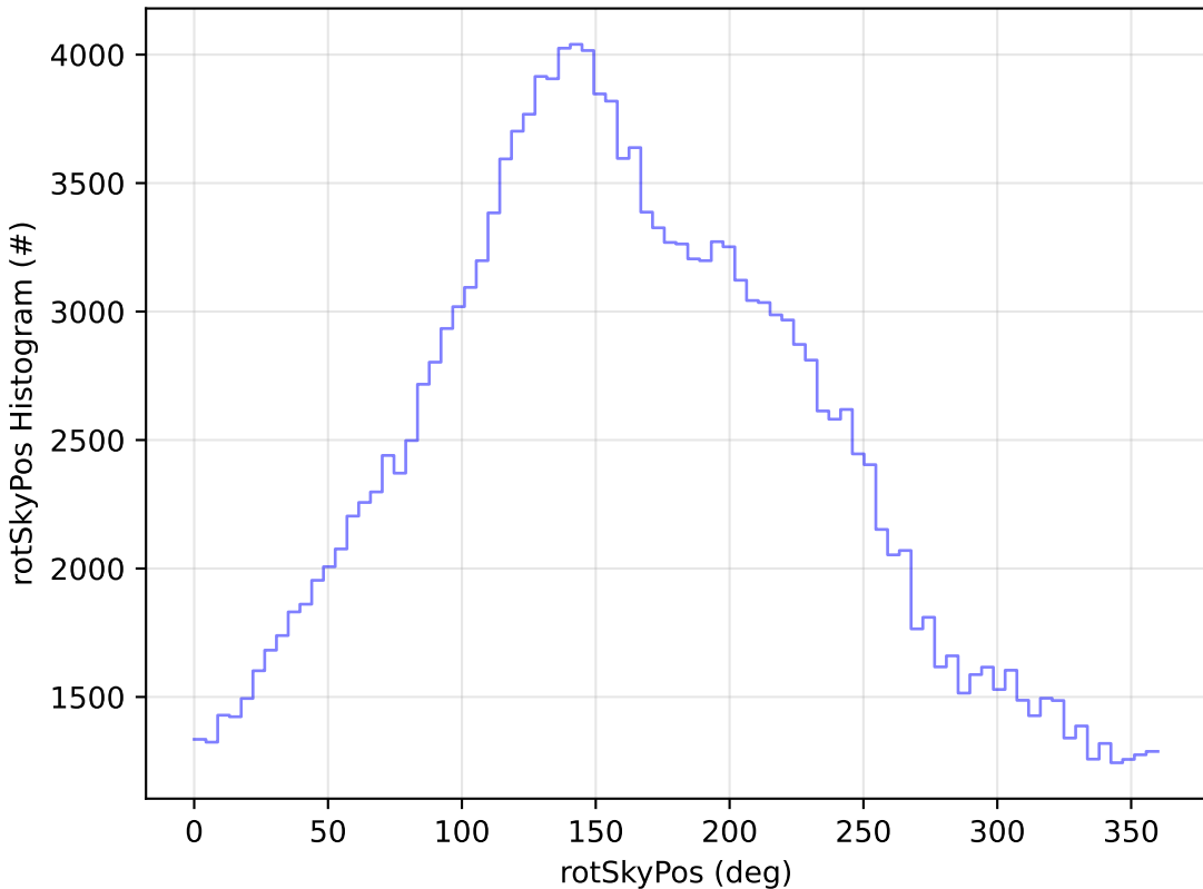
noroll_v3.4_10yrs All sky g band: rotSkyPos Histogram
