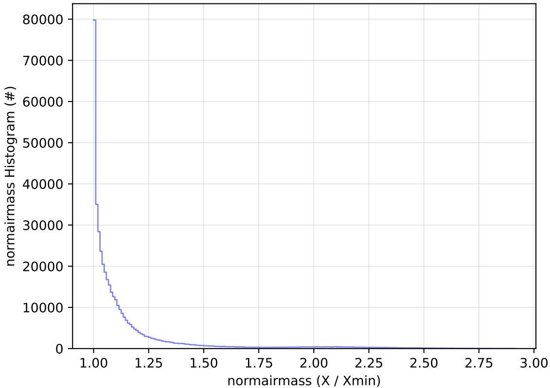
noroll_v3.4_10yrs WFD z band: normairmass Histogram
