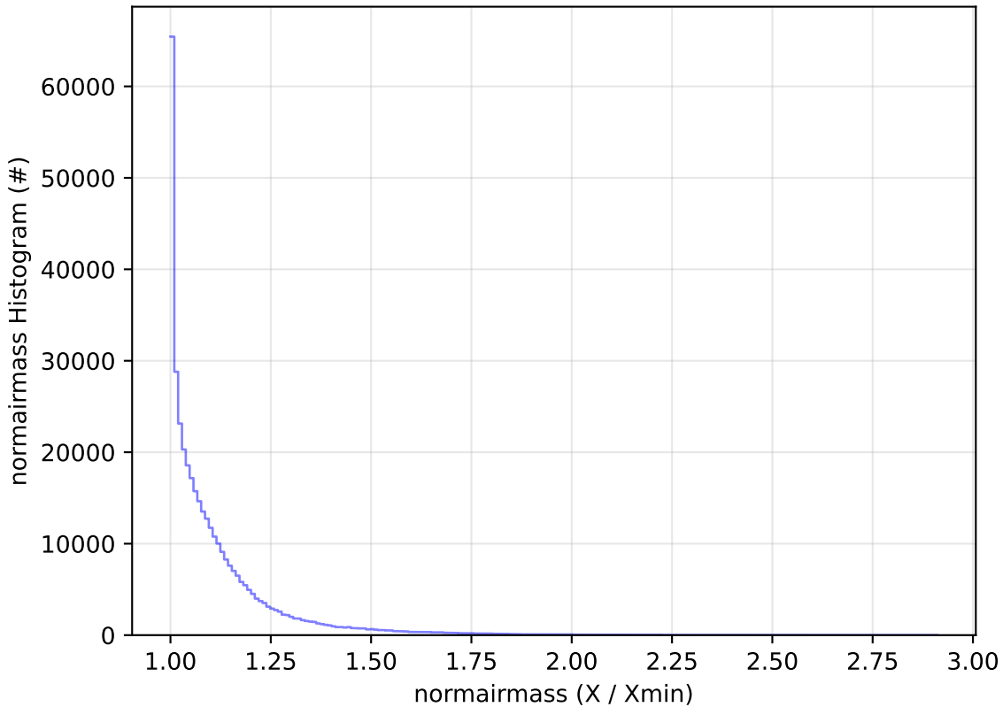
noroll_v3.4_10yrs WFD y band: normairmass Histogram
