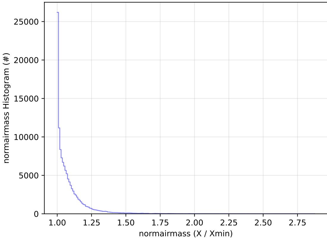
noroll_v3.4_10yrs WFD u band: normairmass Histogram
