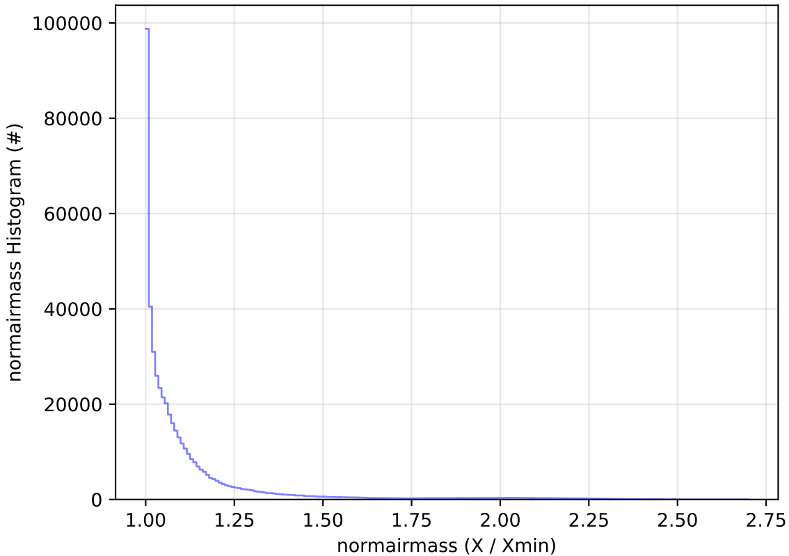
noroll_v3.4_10yrs WFD r band: normairmass Histogram
