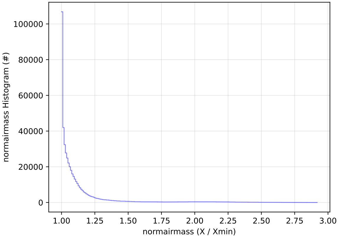
noroll_v3.4_10yrs WFD i band: normairmass Histogram
