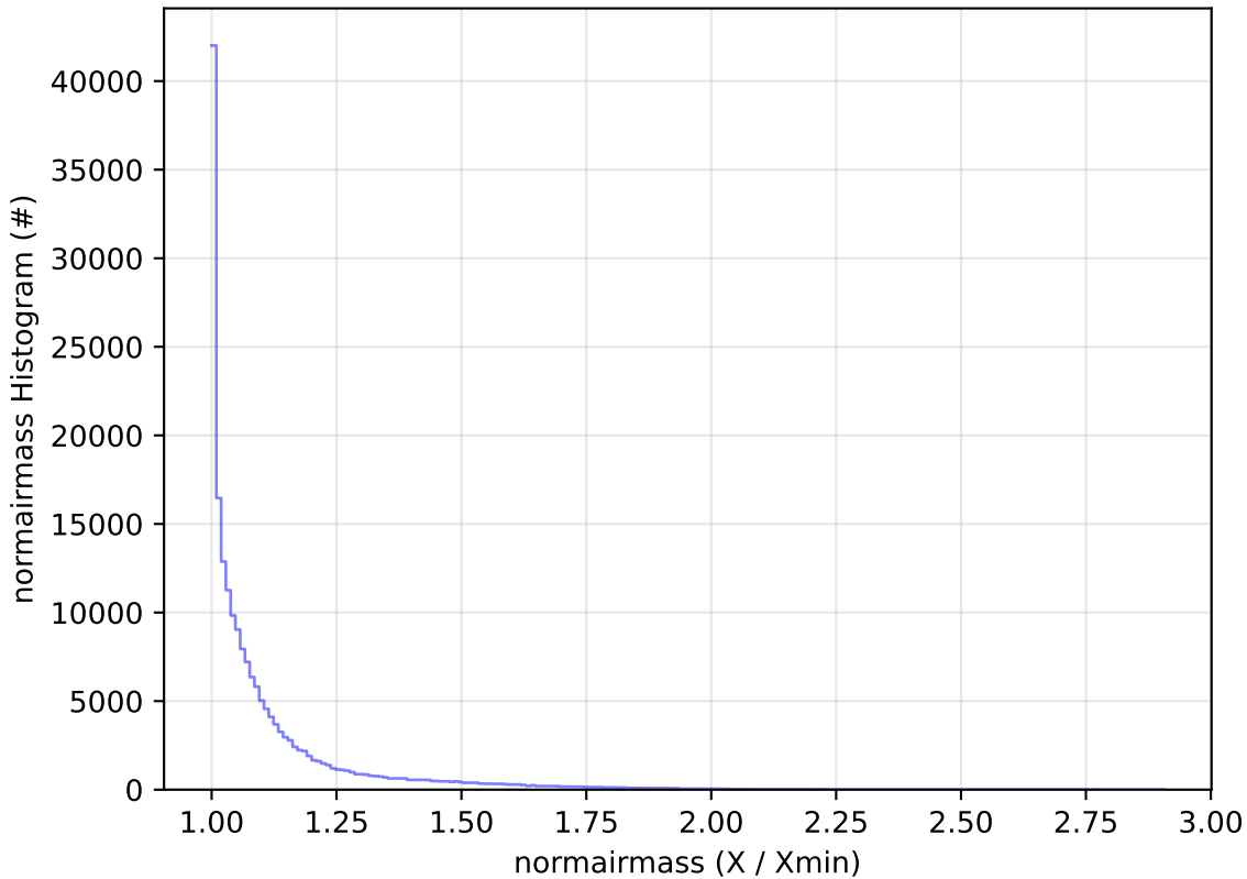
noroll_v3.4_10yrs WFD g band: normairmass Histogram
