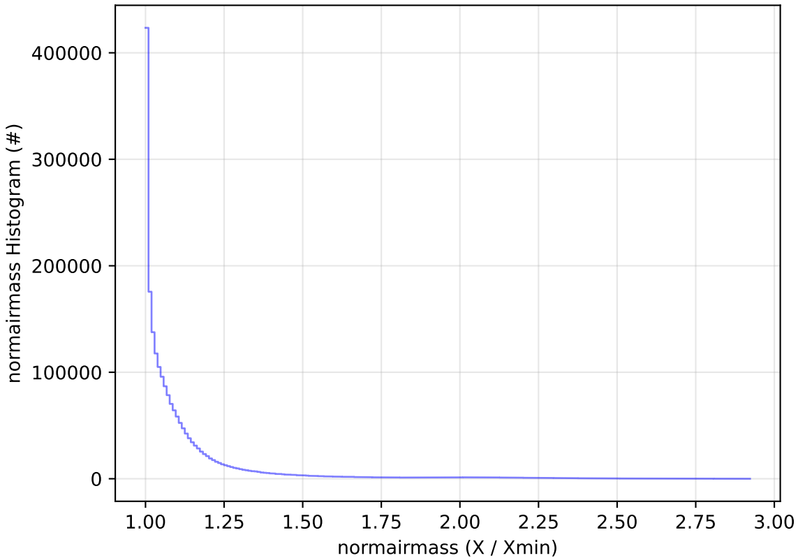
noroll_v3.4_10yrs All sky all bands: normairmass Histogram
