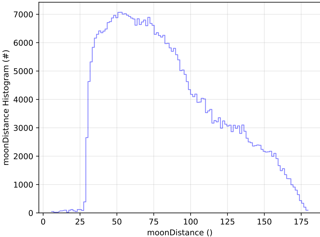
noroll_v3.4_10yrs WFD z band: moonDistance Histogram
