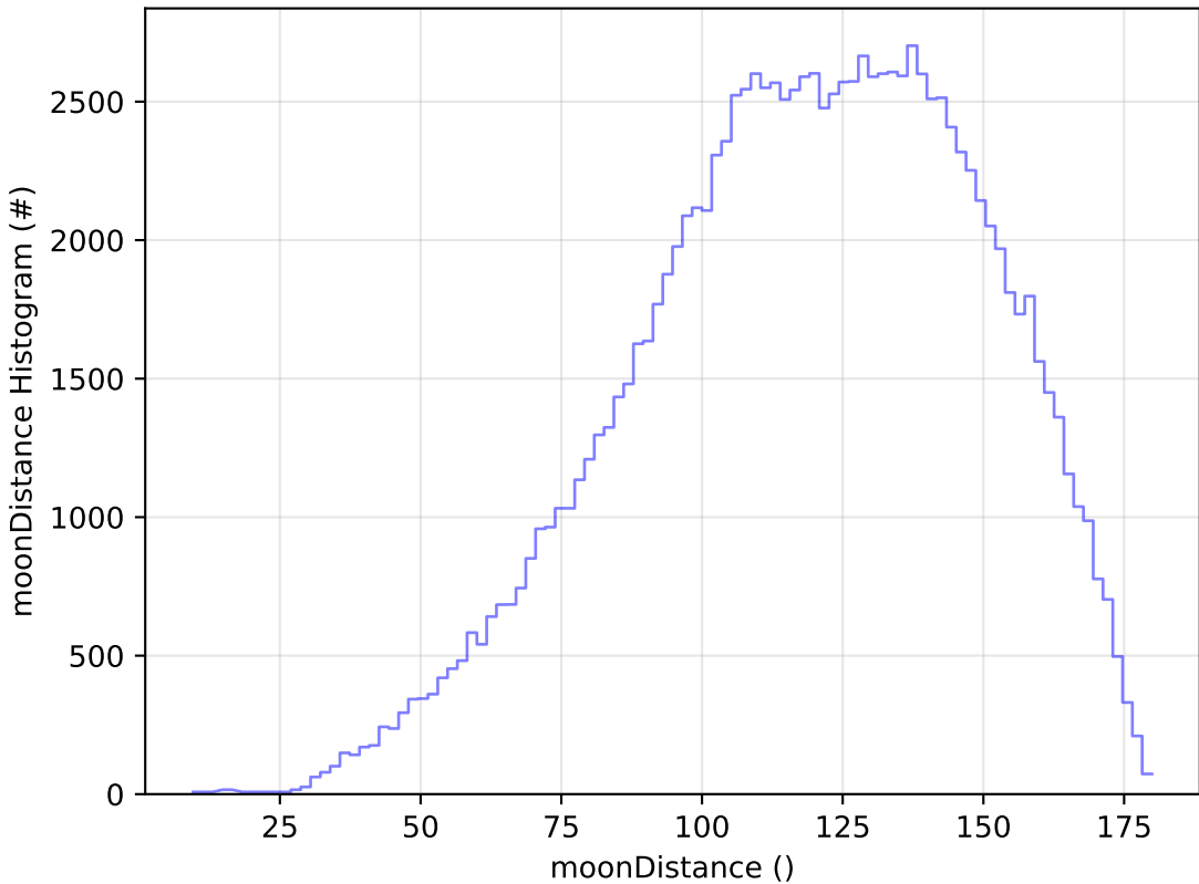
noroll_v3.4_10yrs WFD u band: moonDistance Histogram
