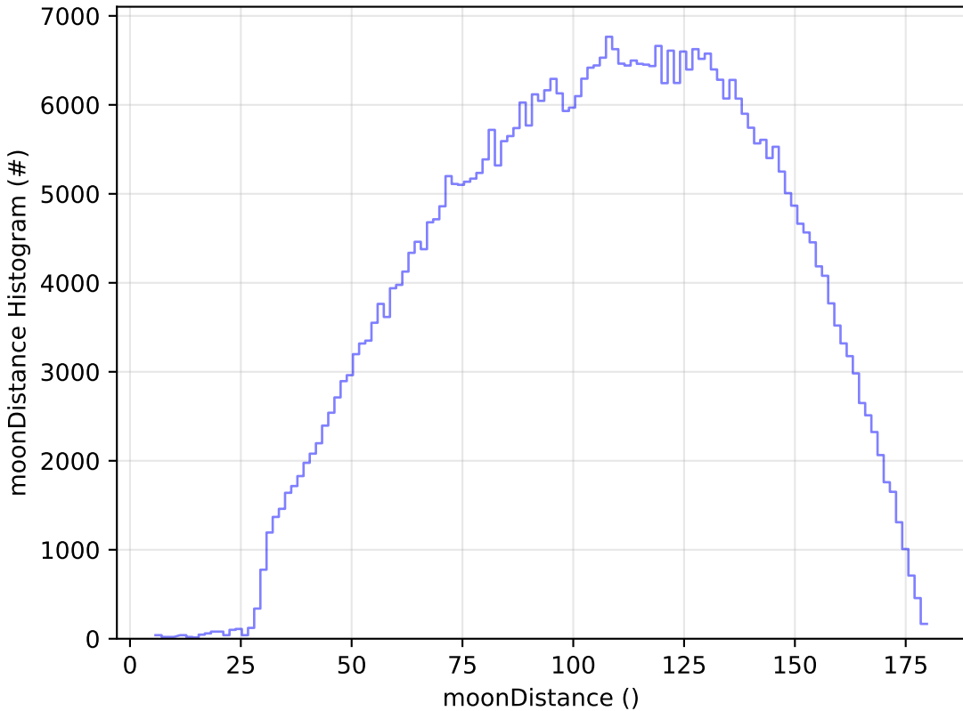
noroll_v3.4_10yrs WFD r band: moonDistance Histogram
