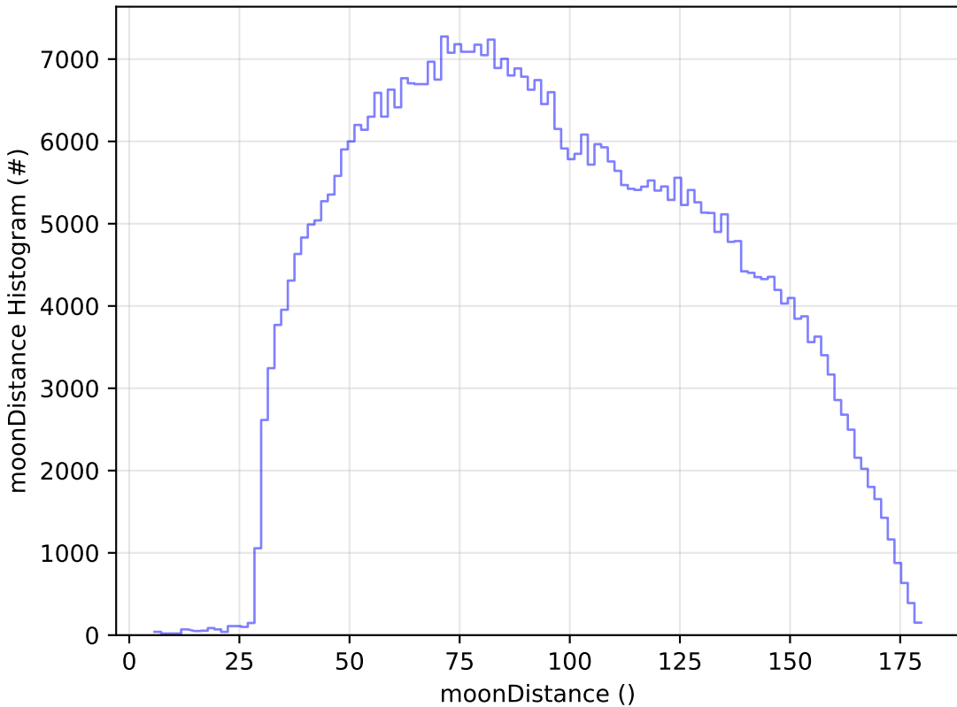
noroll_v3.4_10yrs WFD i band: moonDistance Histogram
