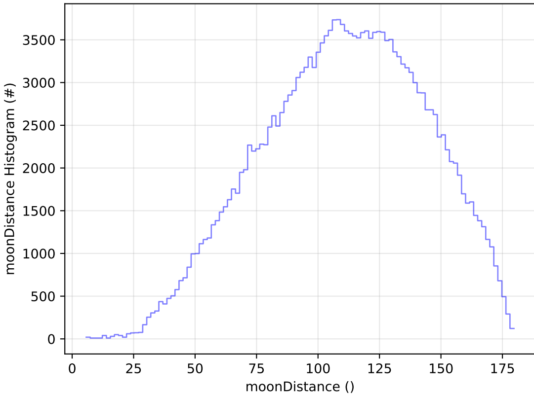
noroll_v3.4_10yrs WFD g band: moonDistance Histogram
