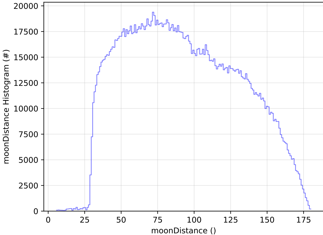
noroll_v3.4_10yrs WFD all bands: moonDistance Histogram
