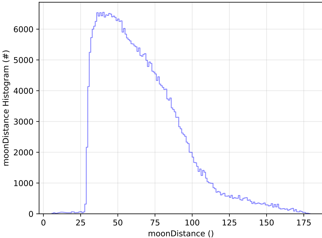
noroll_v3.4_10yrs All sky y band: moonDistance Histogram
