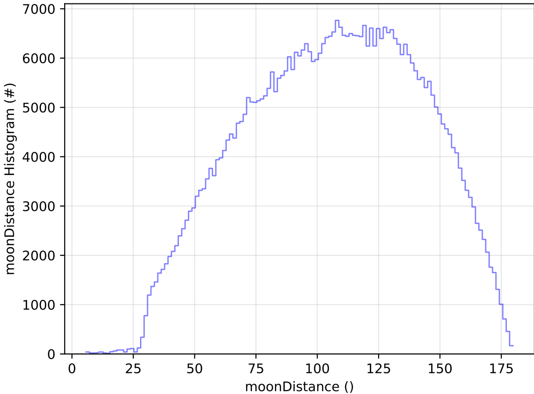
noroll_v3.4_10yrs All sky r band: moonDistance Histogram
