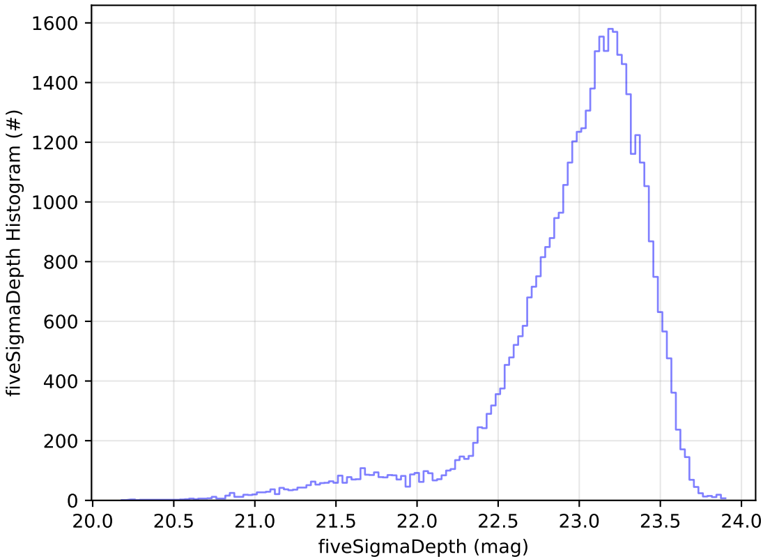
noroll_v3.4_10yrs Yr 1 z band: fiveSigmaDepth Histogram
