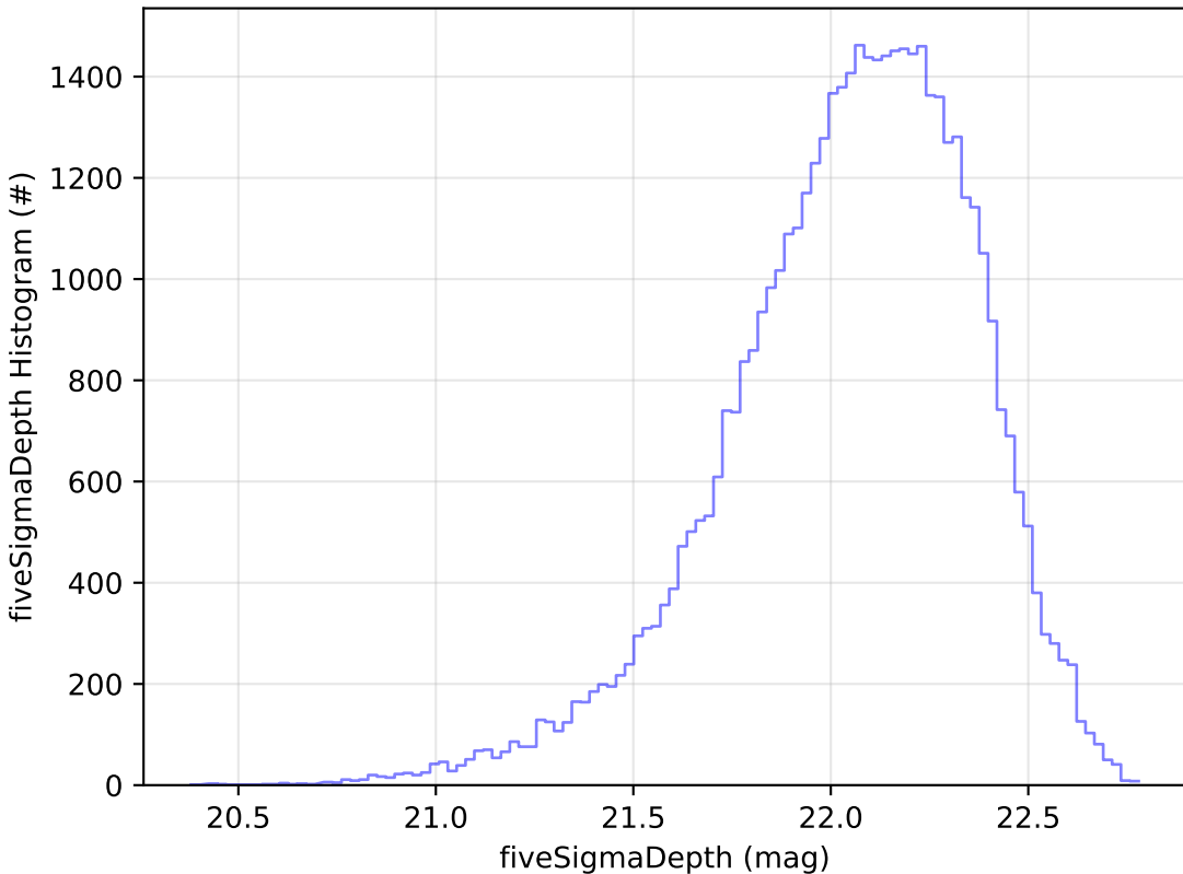
noroll_v3.4_10yrs Yr 1 y band: fiveSigmaDepth Histogram
