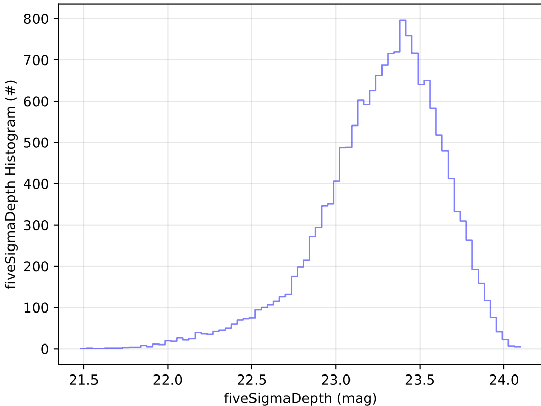
noroll_v3.4_10yrs Yr 1 u band: fiveSigmaDepth Histogram
