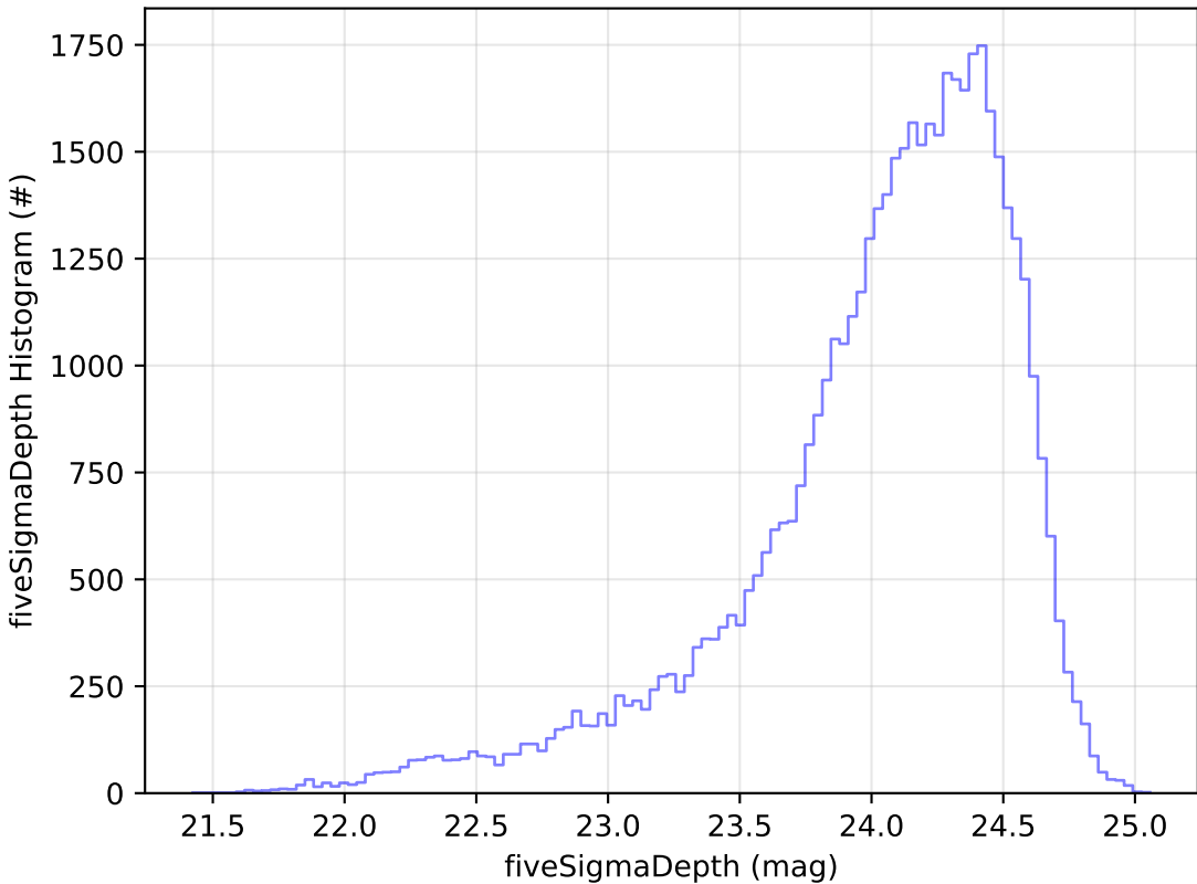
noroll_v3.4_10yrs Yr 1 r band: fiveSigmaDepth Histogram
