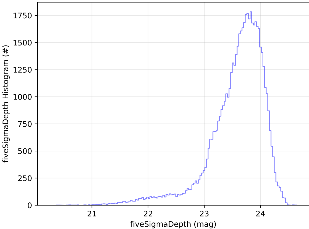
noroll_v3.4_10yrs Yr 1 i band: fiveSigmaDepth Histogram
