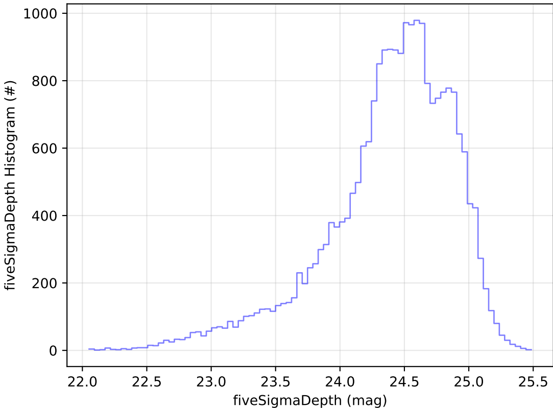
noroll_v3.4_10yrs Yr 1 g band: fiveSigmaDepth Histogram
