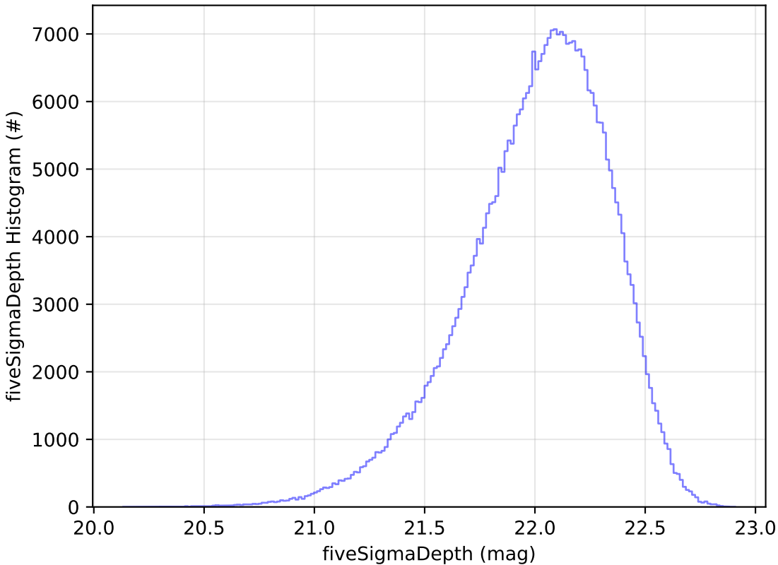
noroll_v3.4_10yrs WFD y band: fiveSigmaDepth Histogram
