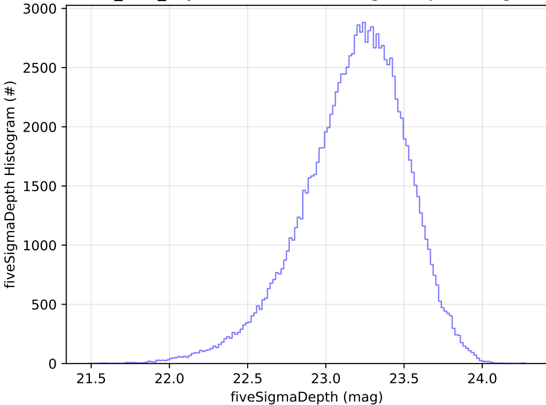
noroll_v3.4_10yrs WFD u band: fiveSigmaDepth Histogram
