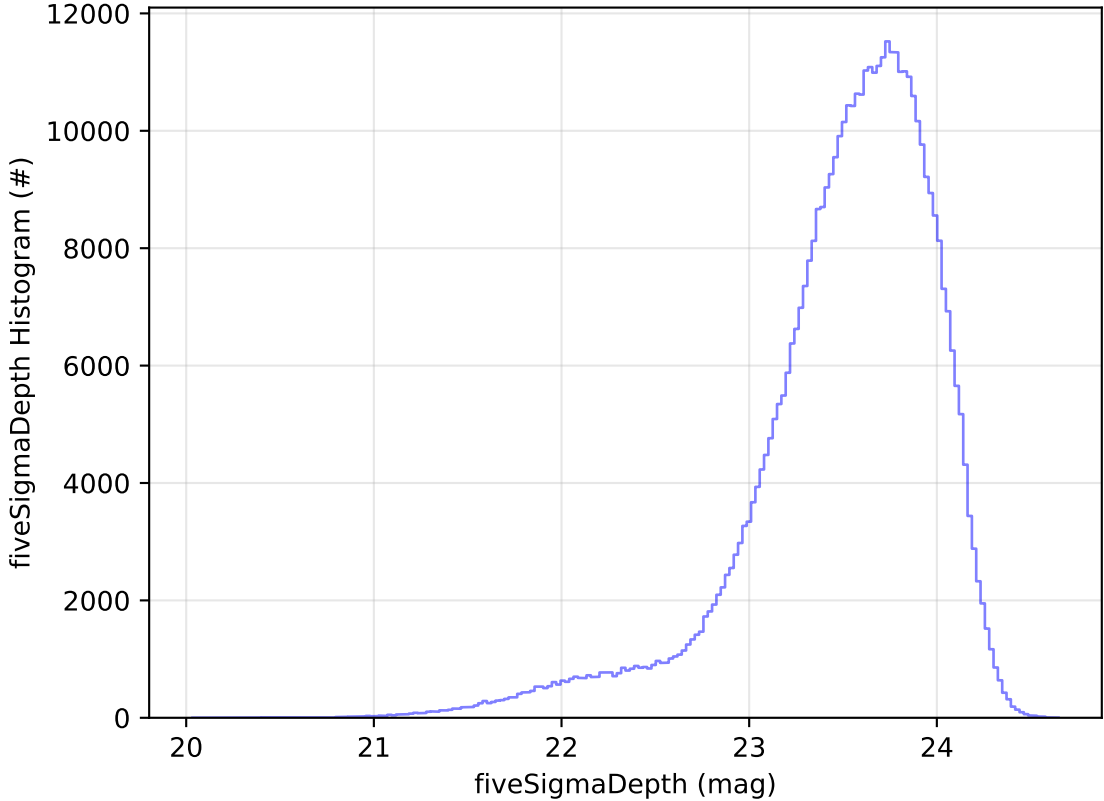
noroll_v3.4_10yrs WFD i band: fiveSigmaDepth Histogram
