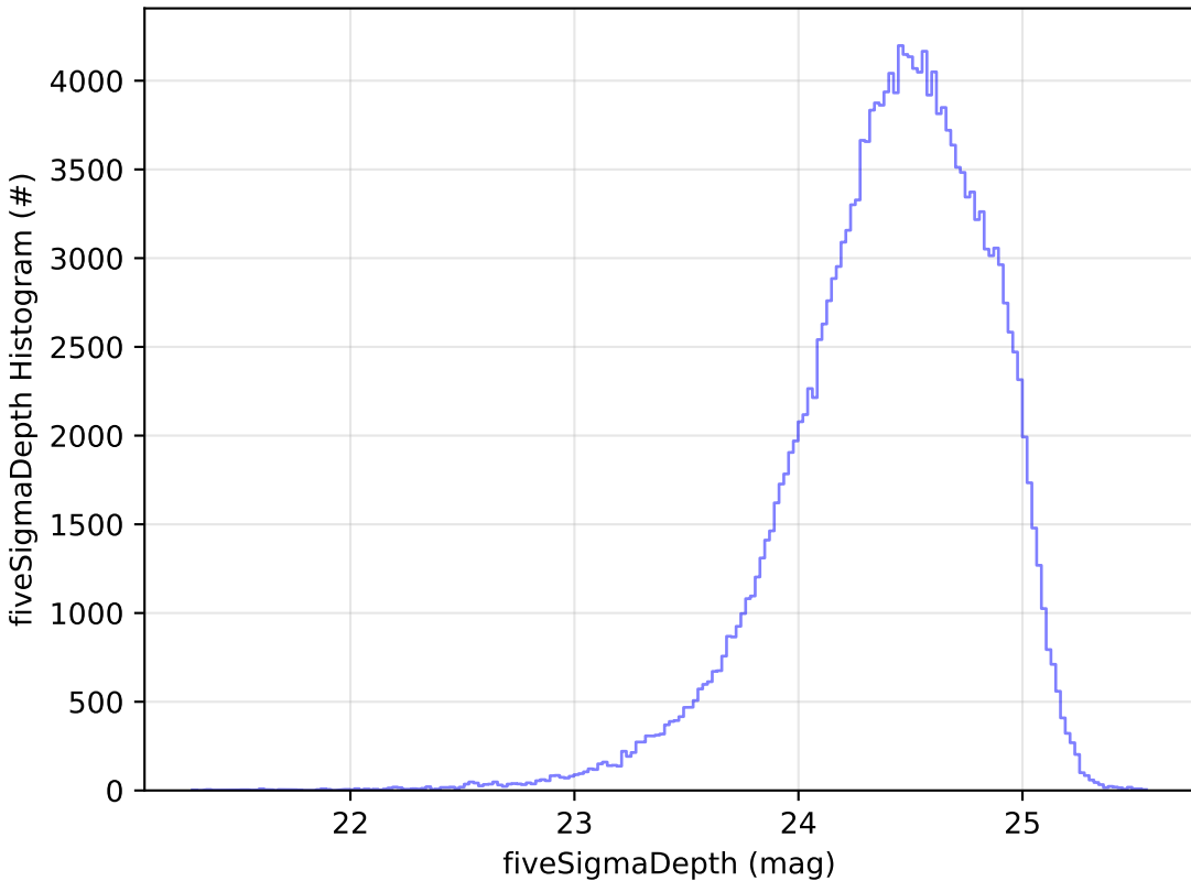
noroll_v3.4_10yrs WFD g band: fiveSigmaDepth Histogram
