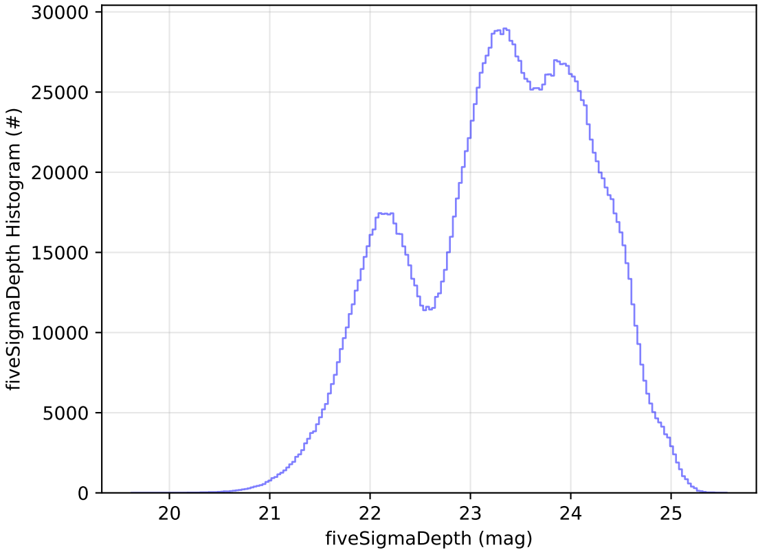
noroll_v3.4_10yrs WFD all bands: fiveSigmaDepth Histogram
