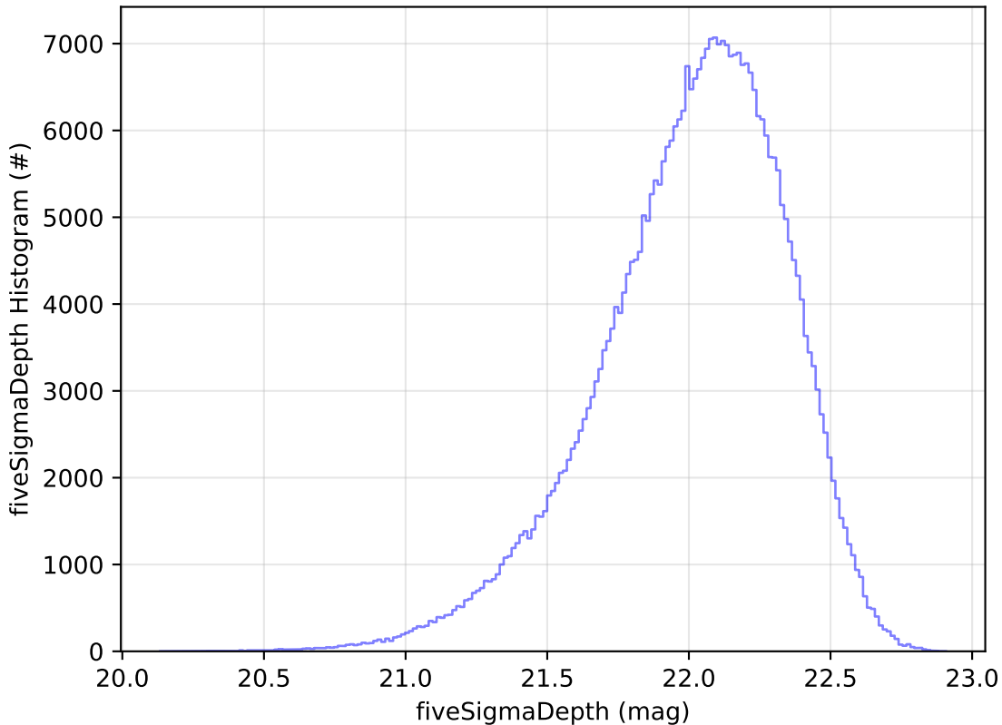
noroll_v3.4_10yrs All sky y band: fiveSigmaDepth Histogram
