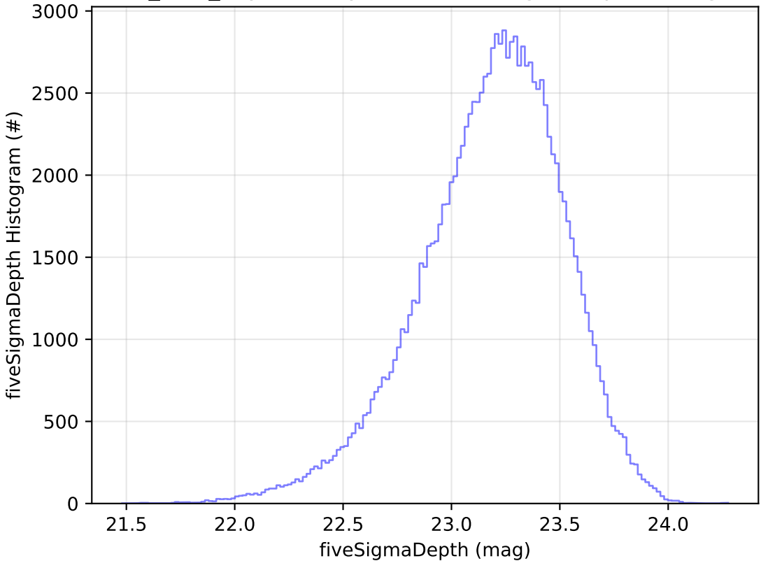
noroll_v3.4_10yrs All sky u band: fiveSigmaDepth Histogram
