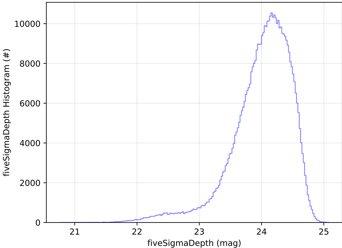
noroll_v3.4_10yrs All sky r band: fiveSigmaDepth Histogram
