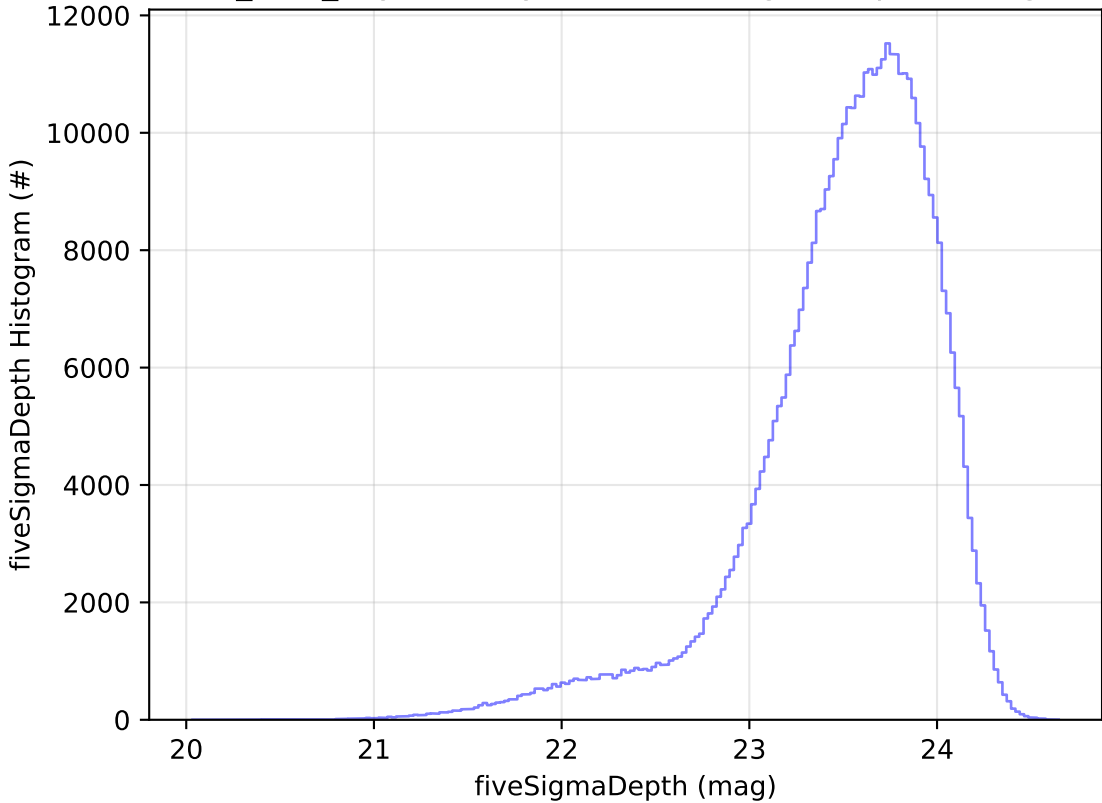
noroll_v3.4_10yrs All sky i band: fiveSigmaDepth Histogram
