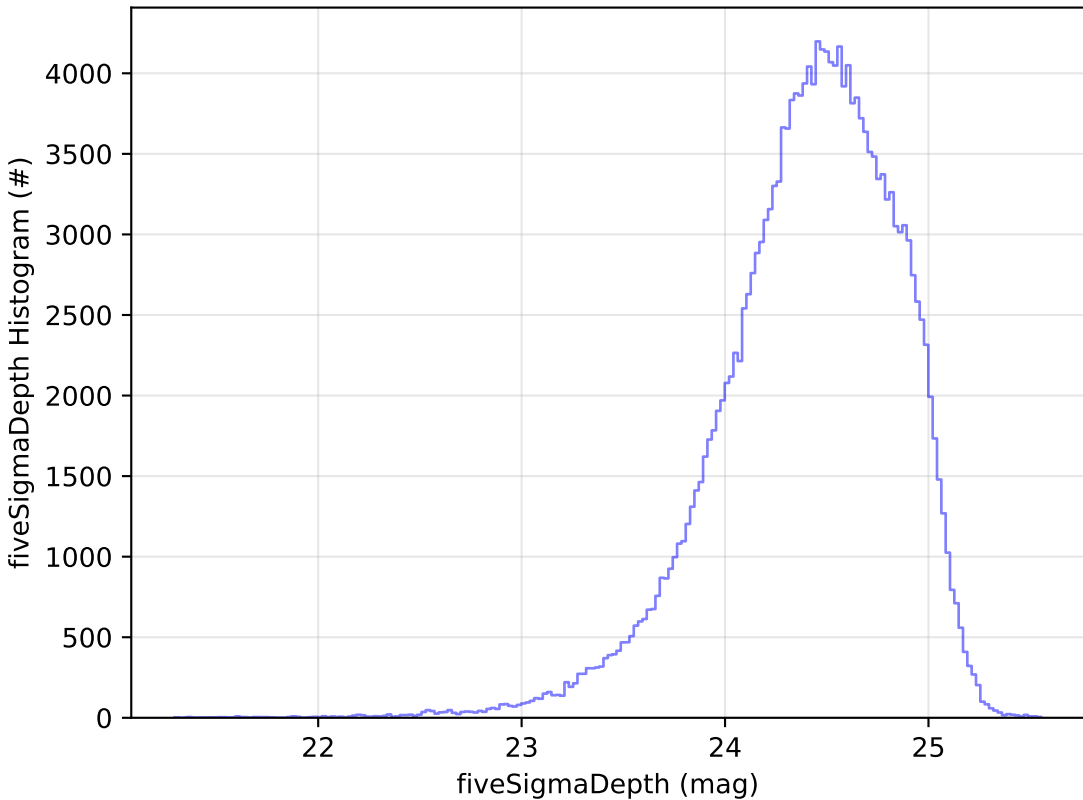
noroll_v3.4_10yrs All sky g band: fiveSigmaDepth Histogram
