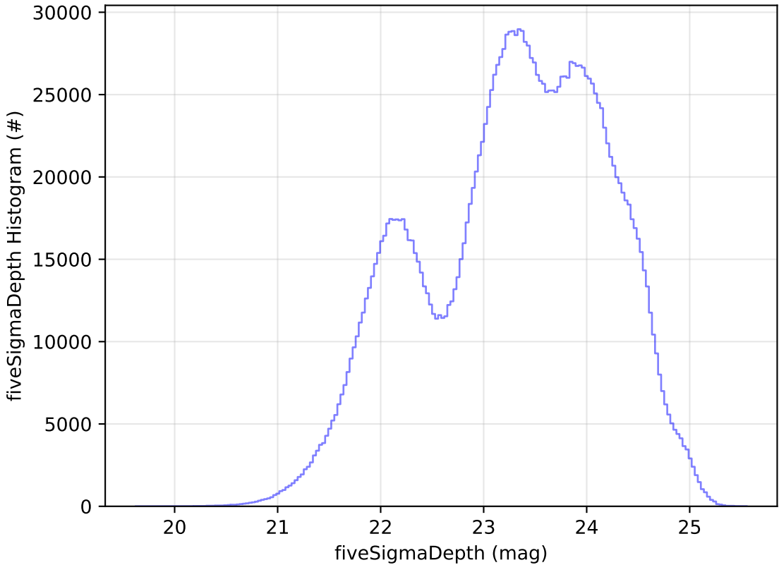
noroll_v3.4_10yrs All sky all bands: fiveSigmaDepth Histogram
