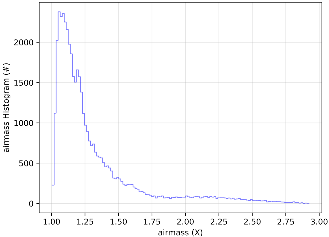
noroll_v3.4_10yrs Yr 1 z band: airmass Histogram
