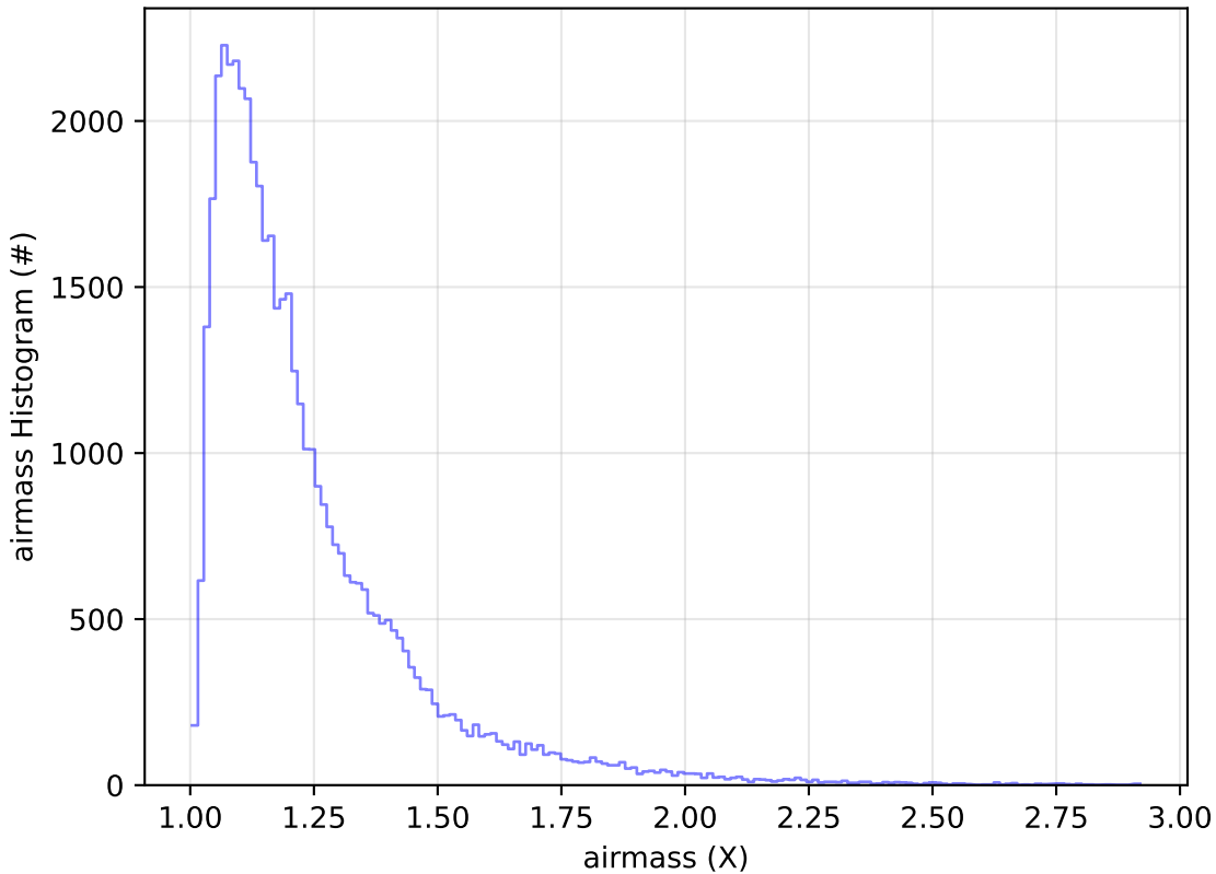
noroll_v3.4_10yrs Yr 1 y band: airmass Histogram
