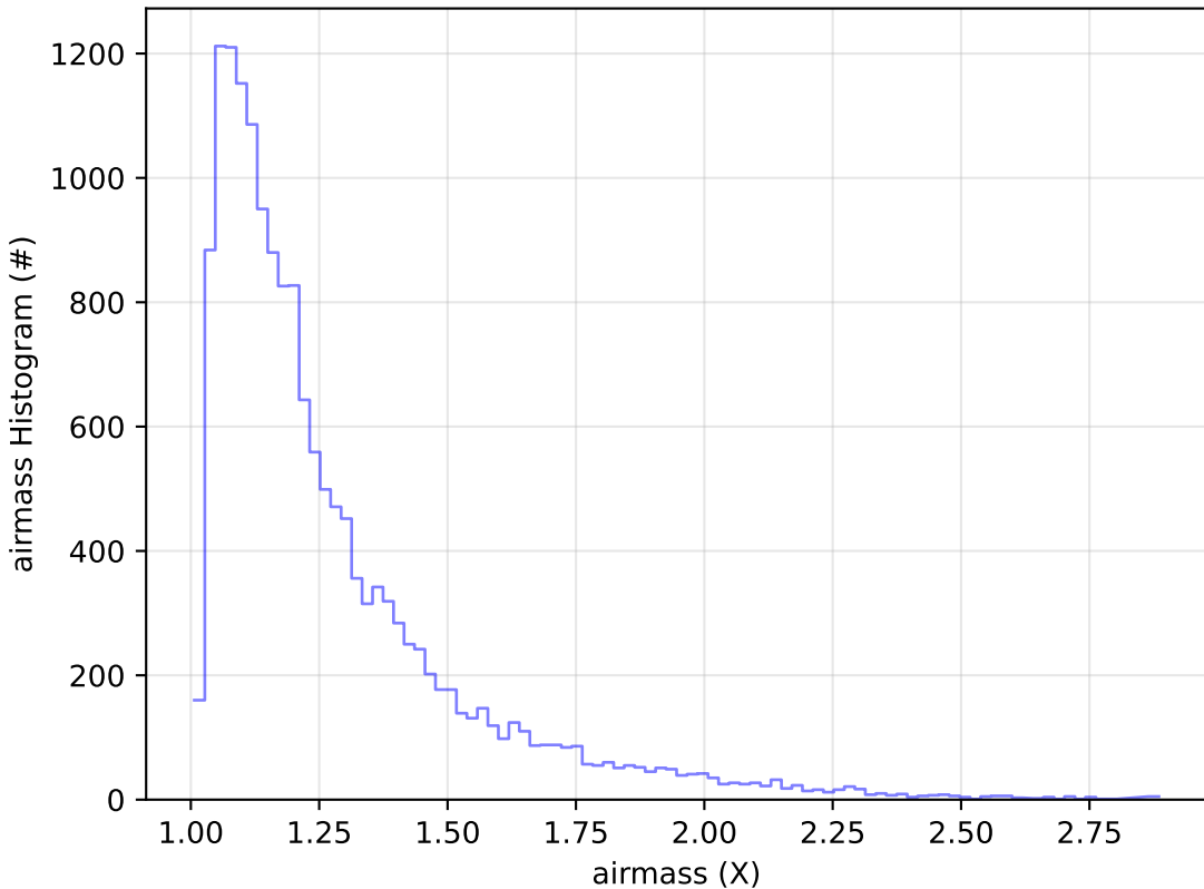
noroll_v3.4_10yrs Yr 1 u band: airmass Histogram
