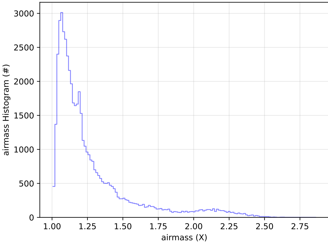
noroll_v3.4_10yrs Yr 1 r band: airmass Histogram
