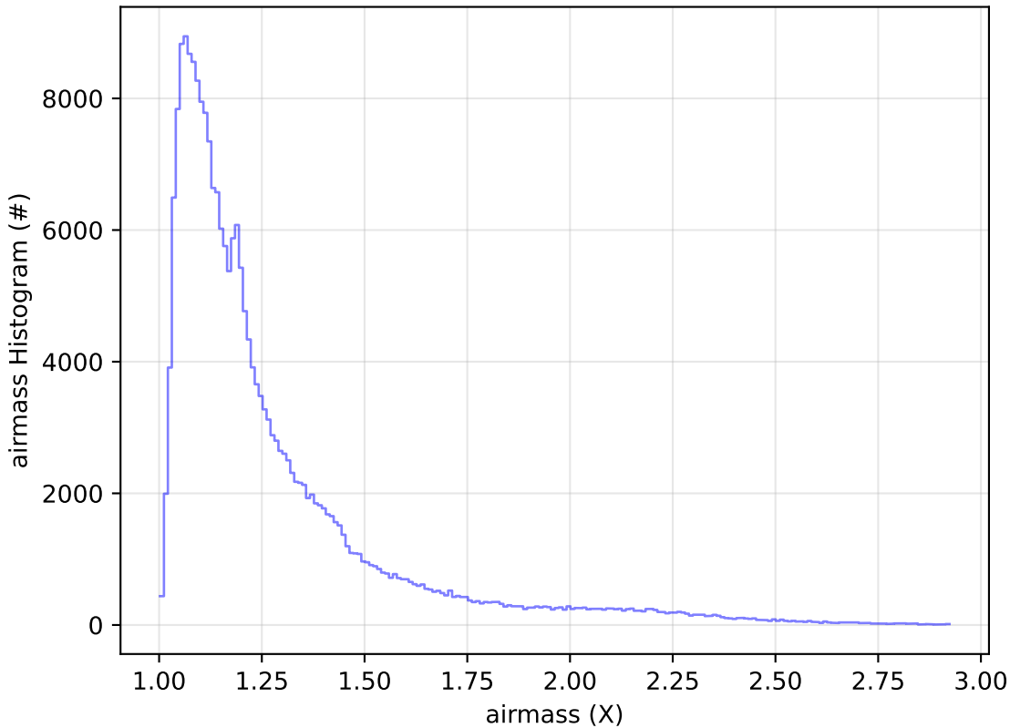
noroll_v3.4_10yrs Yr 1 all bands: airmass Histogram
