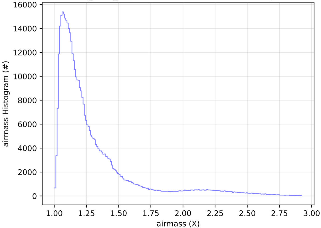
noroll_v3.4_10yrs WFD z band: airmass Histogram
