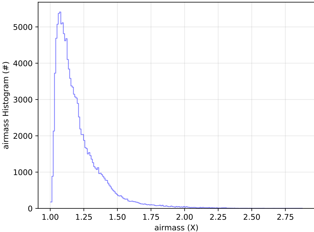
noroll_v3.4_10yrs WFD u band: airmass Histogram
