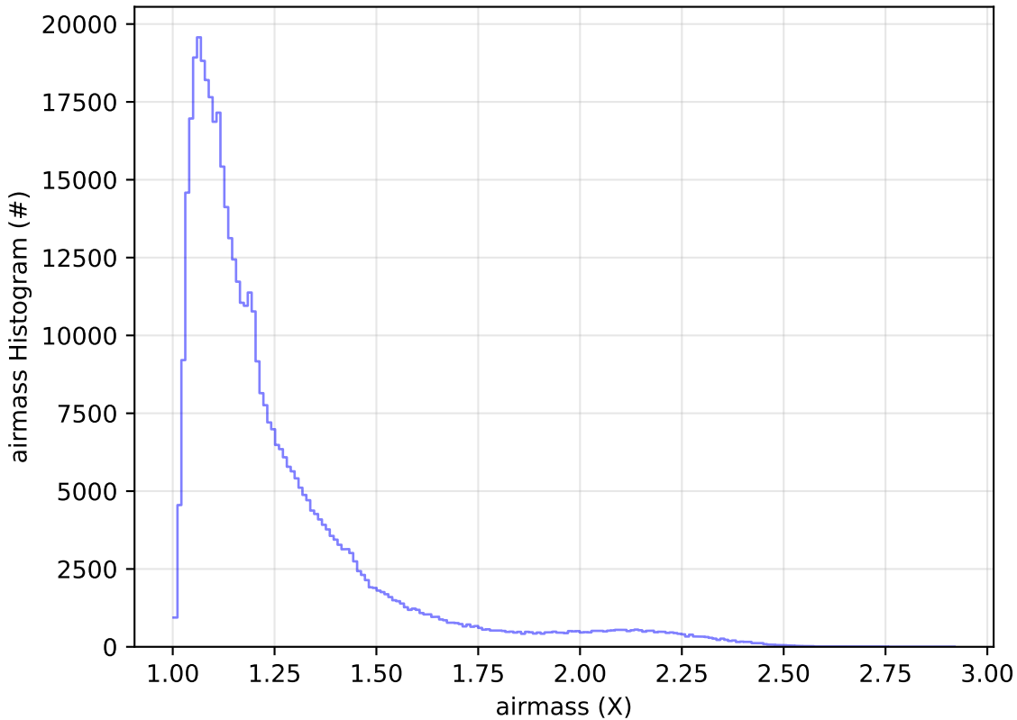
noroll_v3.4_10yrs WFD r band: airmass Histogram
