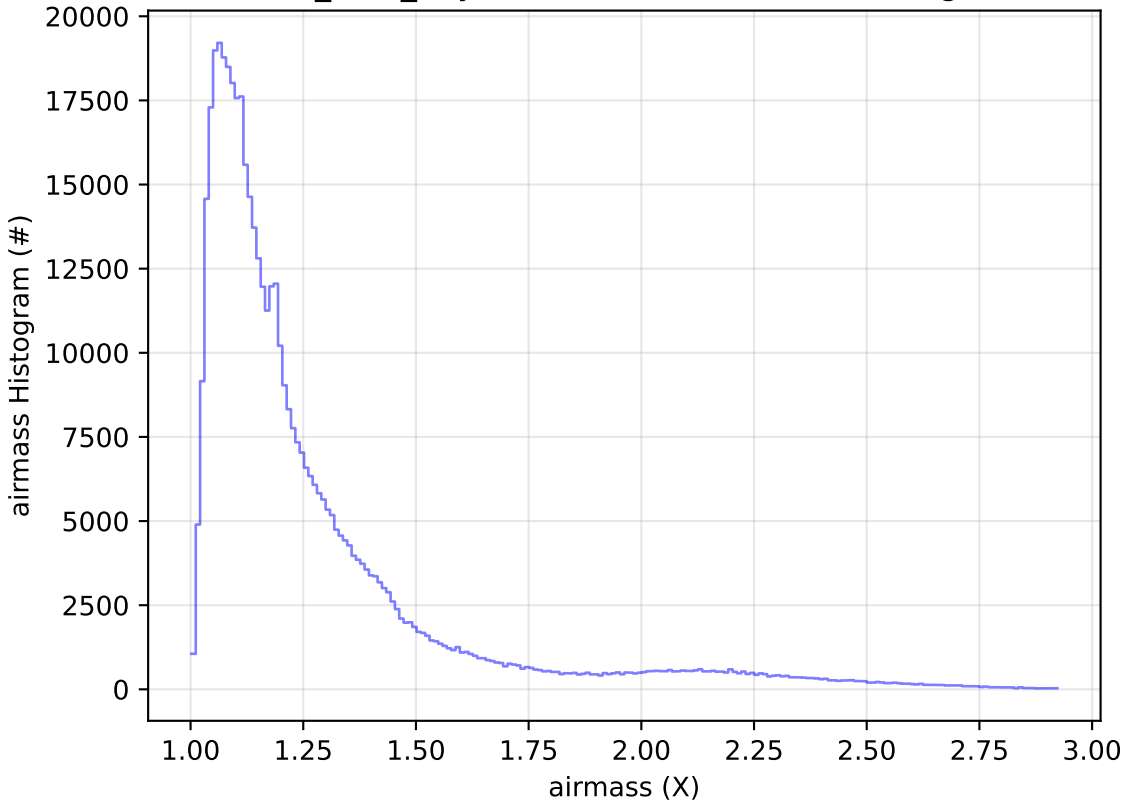
noroll_v3.4_10yrs WFD i band: airmass Histogram
