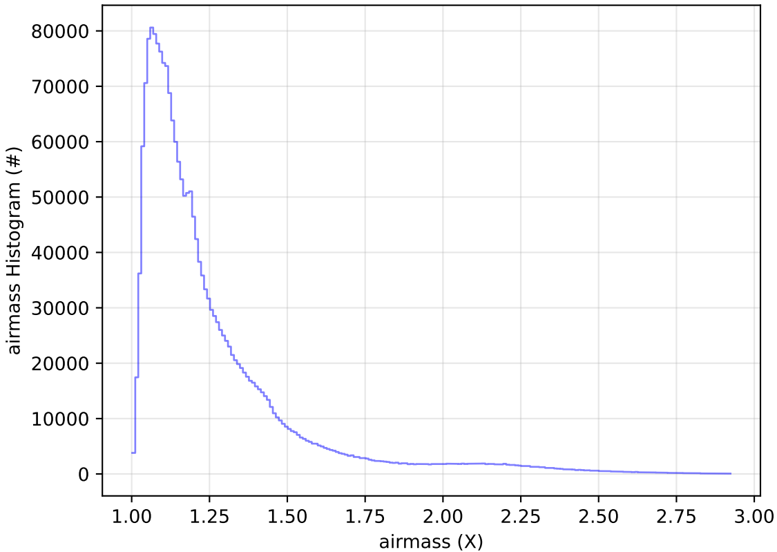
noroll_v3.4_10yrs WFD all bands: airmass Histogram
